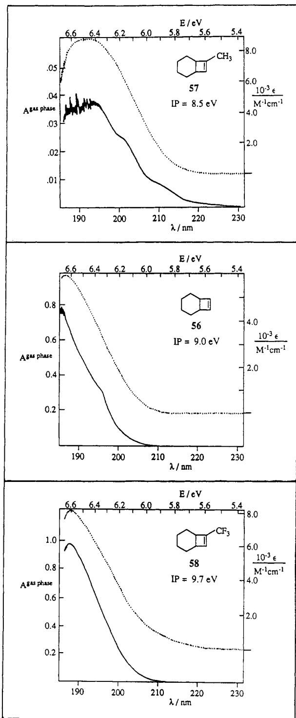
Figure 4. UV absorption spectra of 56–58 in the gas-phase (—) and in deoxygenated pentane solution (....). The left-hand axes refer to the gas-phase spectra, and the right-hand axes refer to the solution phase spectra. Reprinted from ref 73. Copyright 1991 American Chemical Society.
